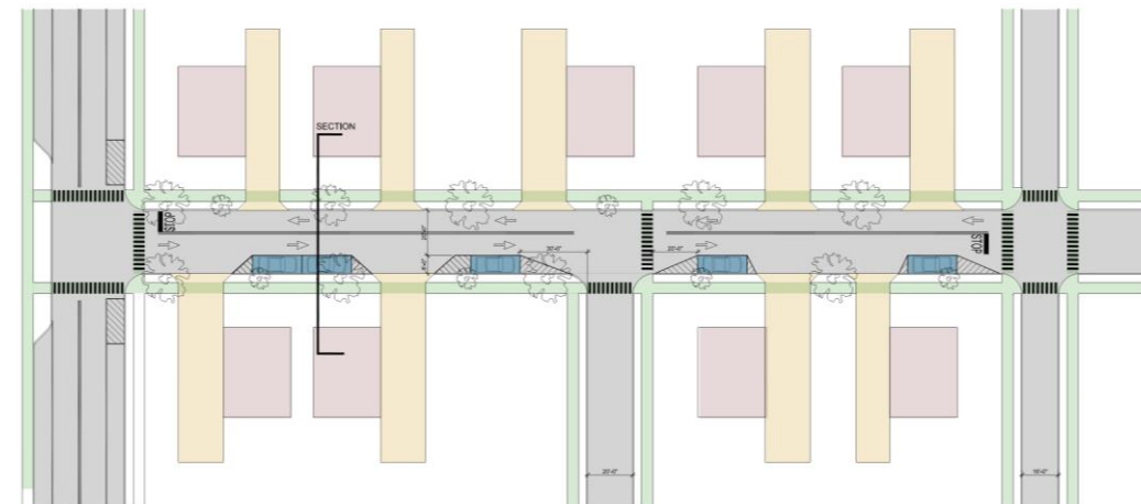
TWO WAY NEIGHBORHOOD STREET WITH ON-STREET PARKING
