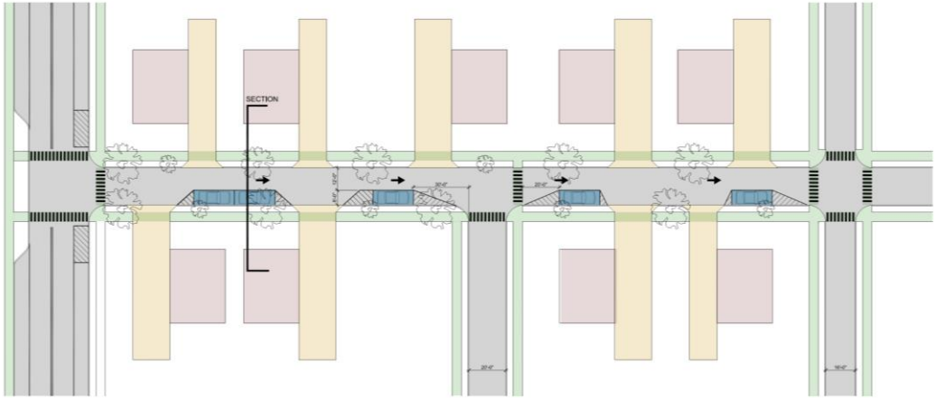
ONE WAY NEIGHBORHOOD STREET WITH ON-STREET PARKING
