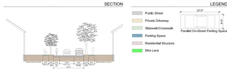
ONE WAY NEIGHBORHOOD STREET WITH ON-STREET PARKING & BIKE LANE
