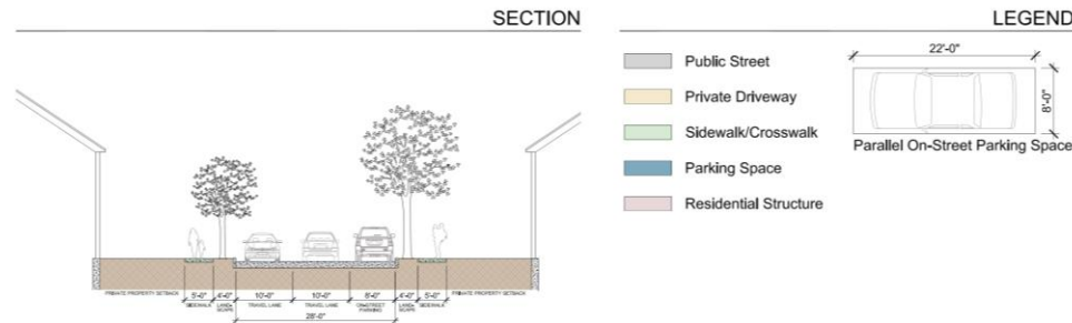
TWO WAY NEIGHBORHOOD STREET WITH ON-STREET PARKING
